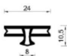
Brtva BR.04
