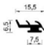
Brtva E-153
