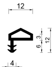
Brtva D-0001
